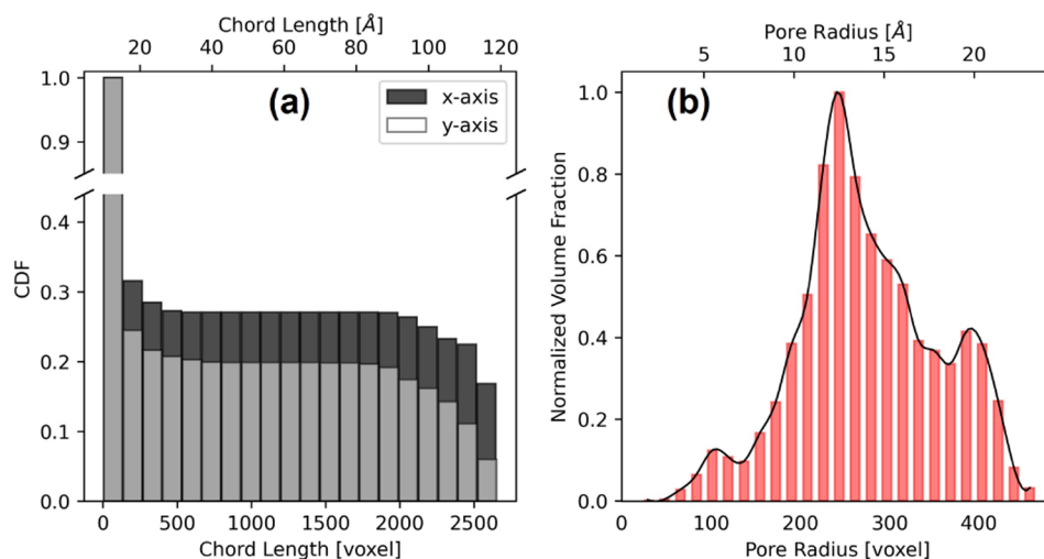
Figure 3. Cumulative distribution function (a) and pore radius histogram (b) calculated for a 64000-atom NPC model using PoreSpy.
